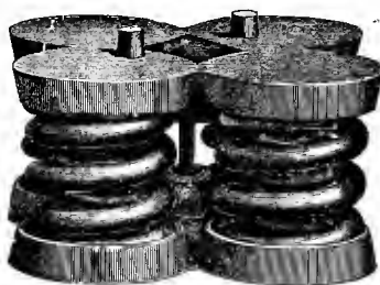
BOLSTER-SPRING, SEATS AND CAPS. NORFOLK & WESTERN RAILROAD. The number of springs depends on capacity of car, each spring being capable of carrying about 10,000 lbs.
